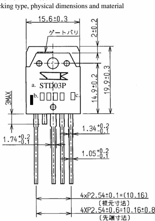
Dimensions between tips
